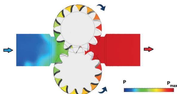
Fig. 101 – Gear pumps delivery principle
