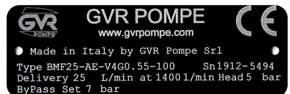
Fig. 203 – Typical nameplate for electric pump
