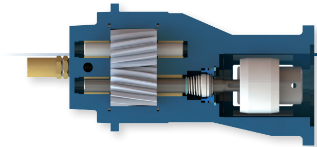
Fig. 301 – APF pump, standard version
