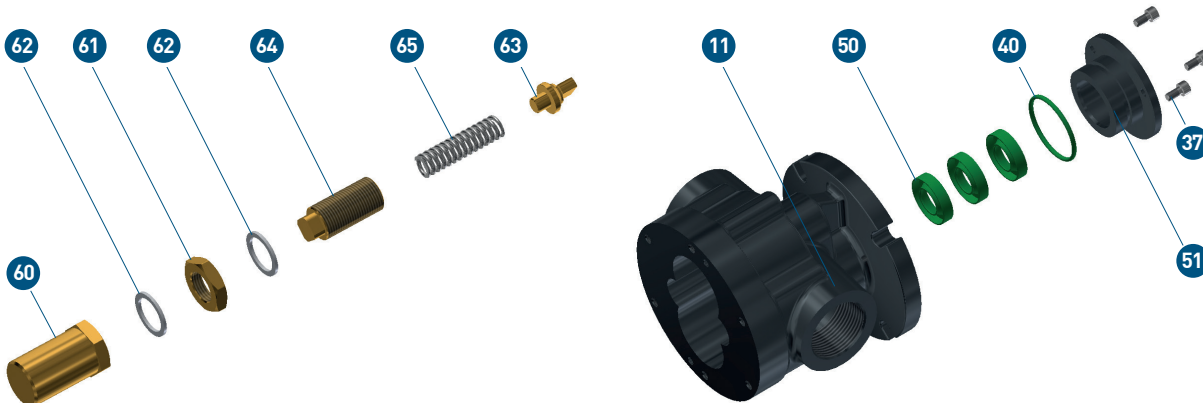
Fig. 308 – Pressure relief valve details
